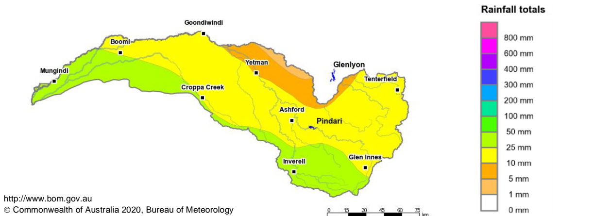
Figure 1: Rainfall totals for the last 30 days (2 Sept to 1 Oct 2020)
