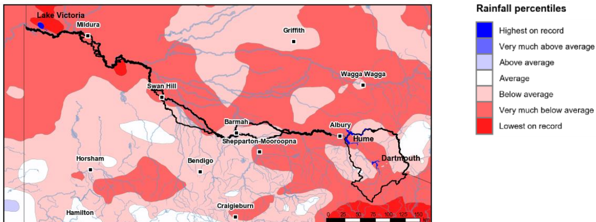
Figure 2: Rainfall percentiles since January 2017 (Compared to 1900-2019 long-term average) (Jan 2017 to Sept 2020) Note: Rainfall percentiles for the period from January 2017 are shown as the Bureau of Meteorology considers January 2017 to be the start of the current dry period for eastern Australia.
