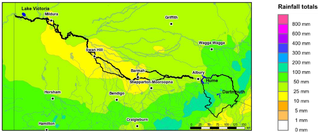
Figure 1: Rainfall totals for the last 30 days (2 Sept to 1 Oct 2020)
