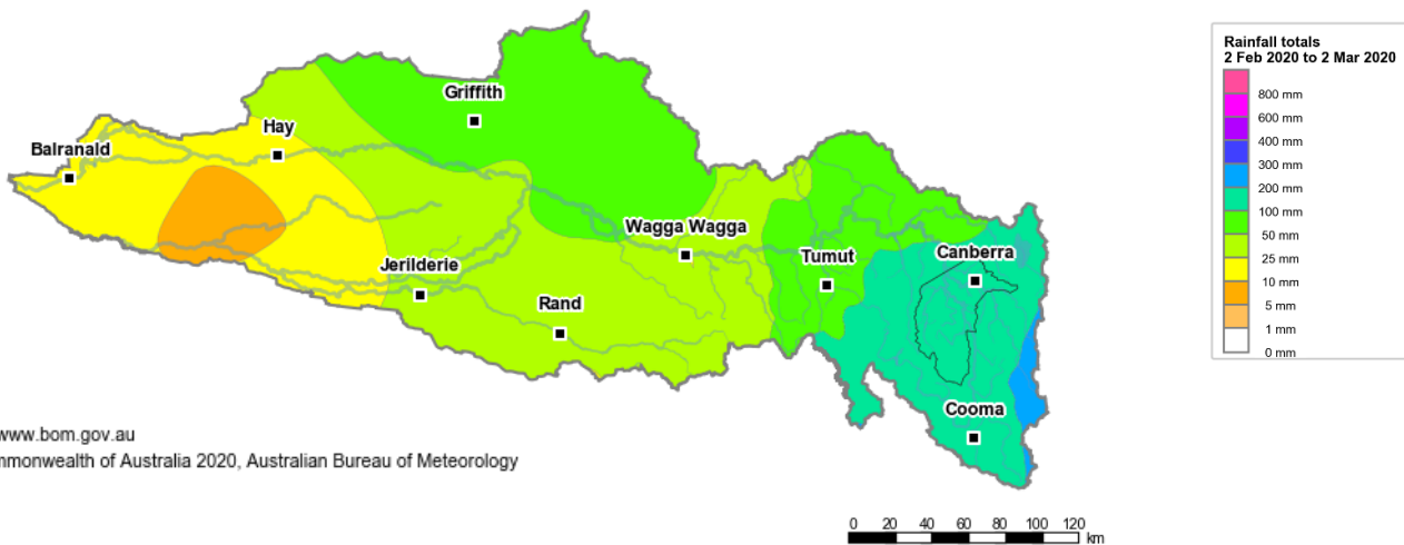
Figure 1: Rainfall totals for the last 30 days
