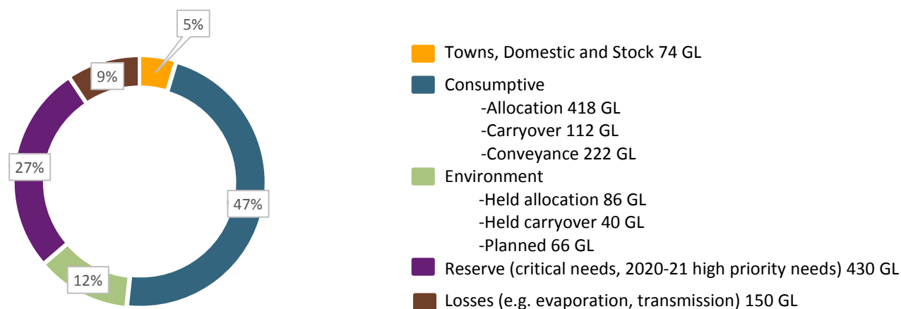
Figure 3: Volumes of water allocated (% of total) for the 2019-20 water year (as at 2 March 2020)
