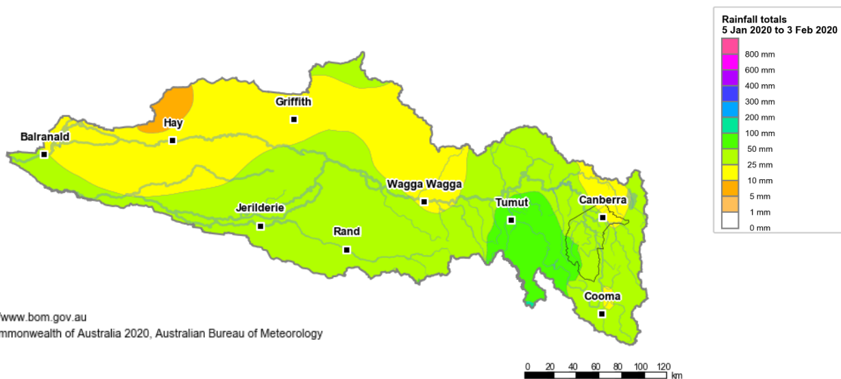
Figure 1: Rainfall totals for the last 30 days
