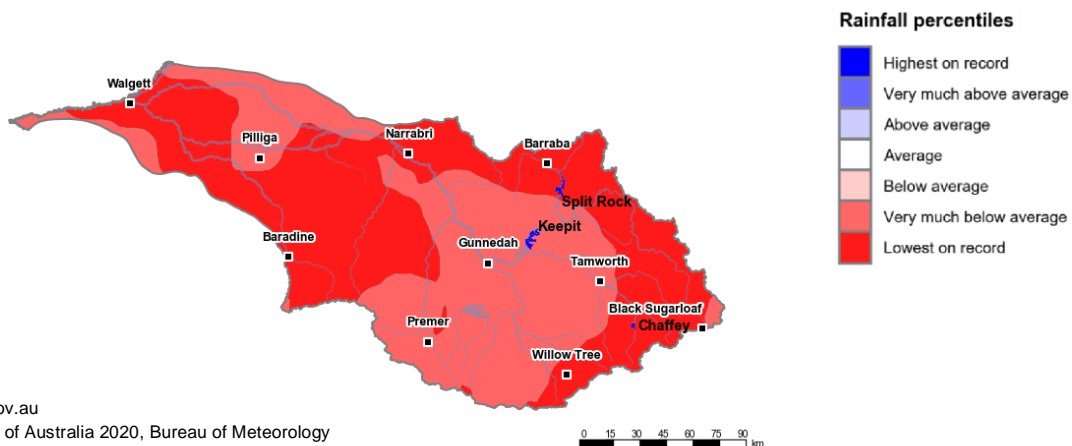
Figure 2: Rainfall percentiles since January 2017 (Compared to 1900-2019 long-term average) (Jan 2017 to May 2020)
