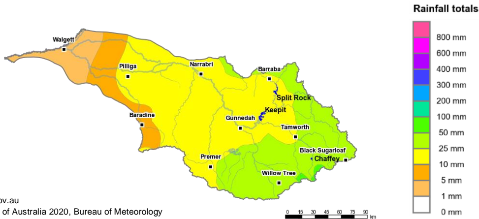
Figure 1: Rainfall totals for the last 30 days (3 May to 1 June 2020)
