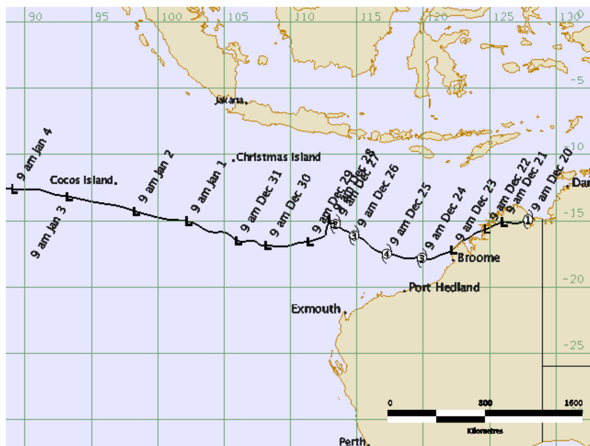
Figure 1. Track of Severe TC Billy 20 December 2008 – 4 January 2009.
