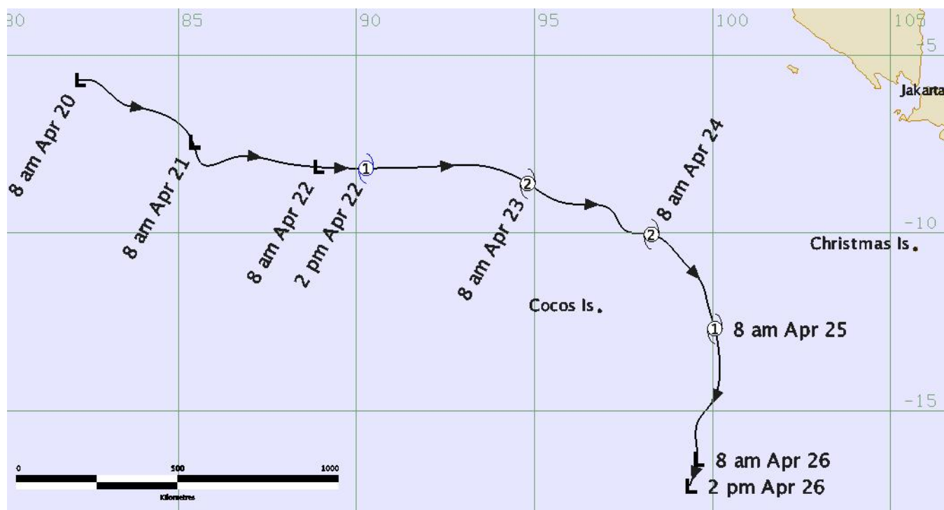
Figure 1. Track of Tropical Cyclone Durga .
