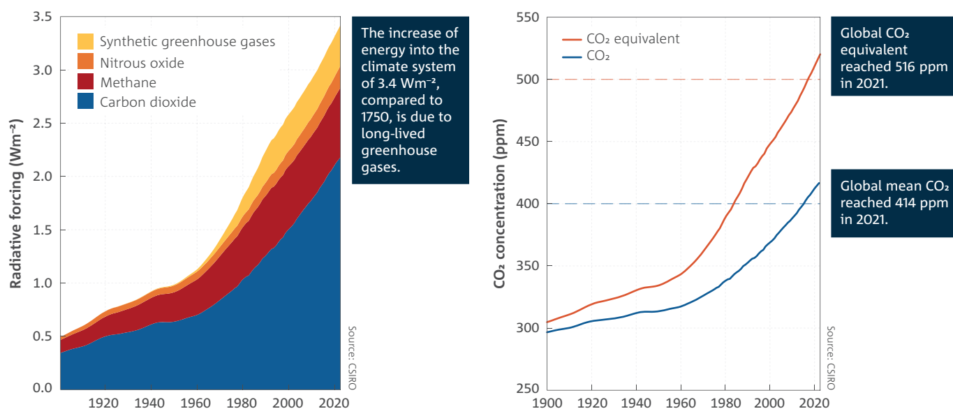
Left: Radiative forcing relative to 1750 due to the long-lived greenhouse gases \text{CO}_2 , methane, nitrous oxide and the synthetic greenhouse gases, expressed as watts per metre squared. Right: Global mean \text{CO}_2 concentration and global mean greenhouse gas concentrations expressed as \text{CO}_2 -e (ppm). \text{CO}_2 -e is calculated from the atmospheric concentrations of \text{CO}_2 , methane, nitrous oxide and the suite of synthetic greenhouse gases.
