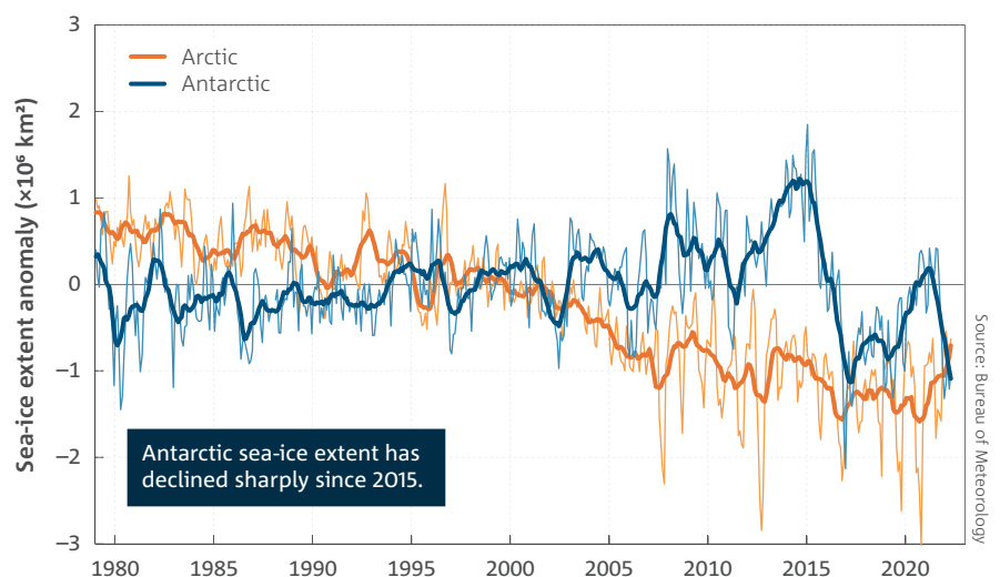
Antarctic and Arctic sea-ice extent (shown as the anomaly relative to 1981–2010) for January 1979 to April 2022 ( 10^6 \text{ km}^2 ). Thin lines are monthly averages and indicate the variability at shorter timescales, while thick lines are 11-month moving averages (centred)—tapered towards end-points.
