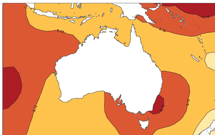
Trends in sea surface temperature in the Australian region (4–46°S and 94–174°E) from 1950–2021.
