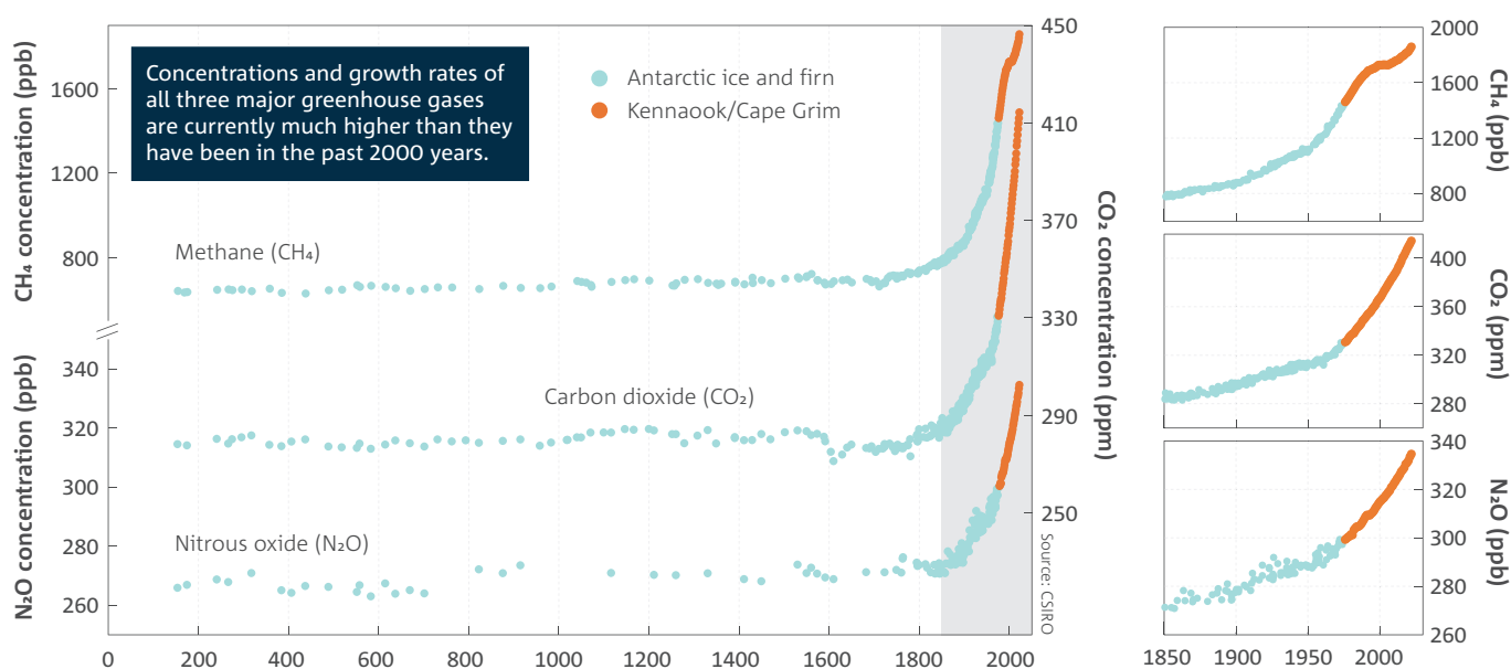
Concentrations of the major greenhouse gases ( \text{CO}_2 , methane and nitrous oxide) in the atmosphere over the past 2000 years. Grey data are measured from air extracted from Antarctic ice cores and the overlying compressed snow (firn) layer. Orange data show the modern in situ record measured at Kennaook/Cape Grim Baseline Air Pollution Station. Note the different scales used for the concentration of each gas.
